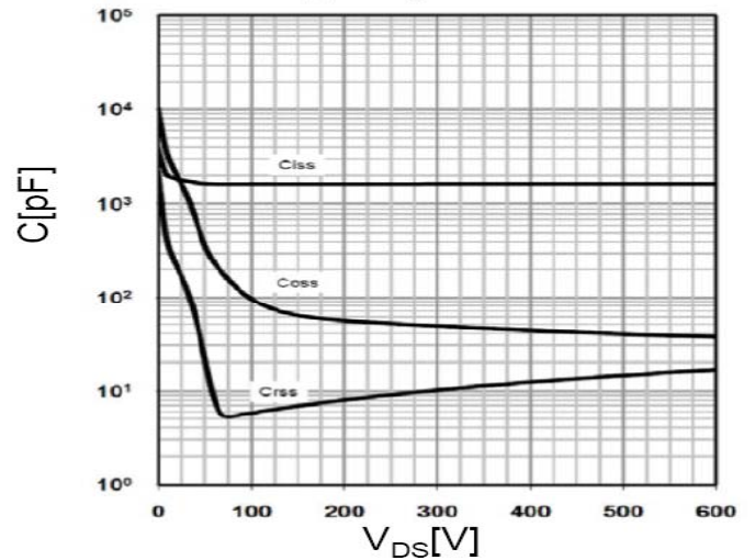
Capacitance
