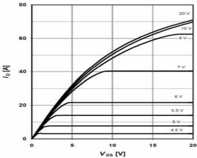
Output Characteristic
