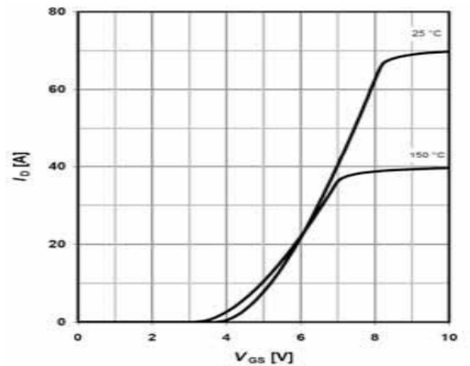
Transfer Characteristic
